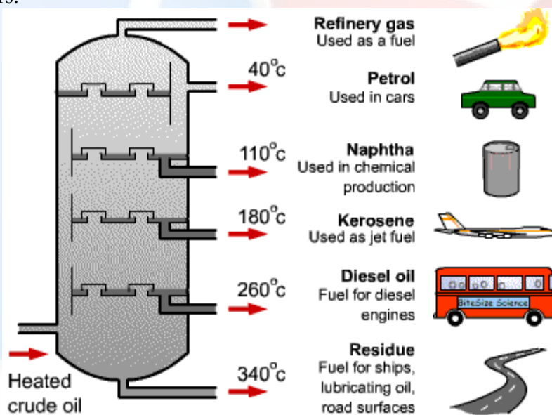
Fig. 1.14 Fractionating column
