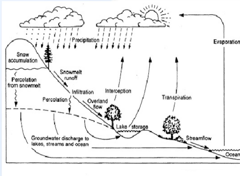
Fig.1.1 Water Cycle
