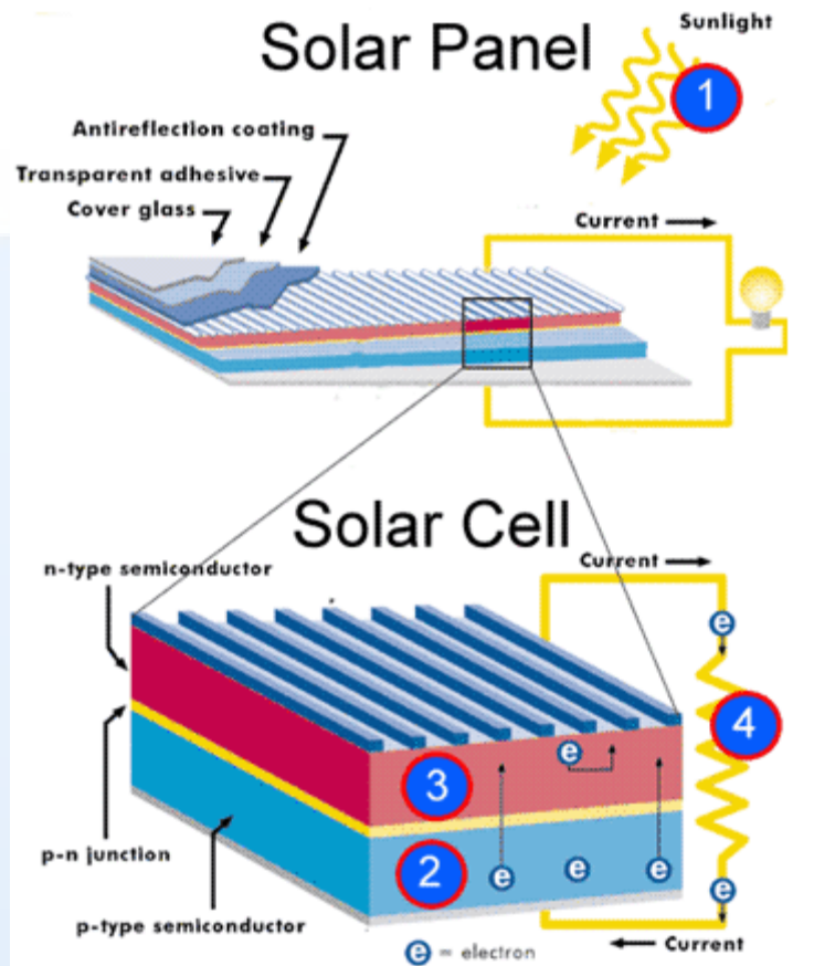
Fig.1.7 Solar cell
