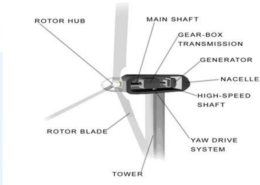
Fig. 1.9 Wind mill
