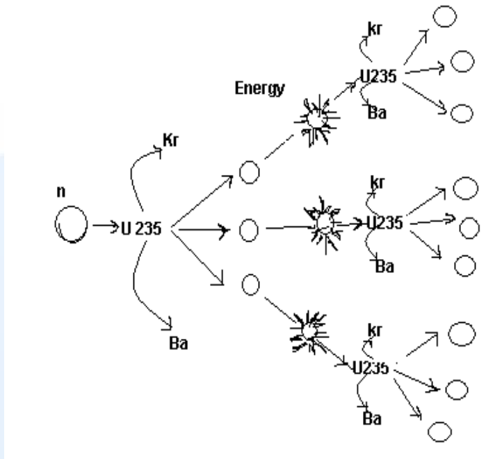
Fig. 1.15 Nuclear fission-chain reaction
